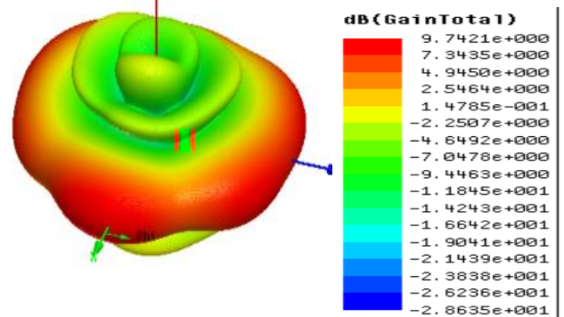
Fig.10: 3D polar plot with readings
