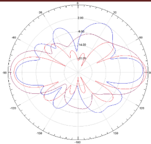
Fig.11.: Radiation pattern
