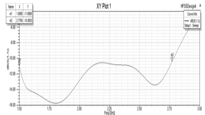
Fig. 9: Reflection coefficient
