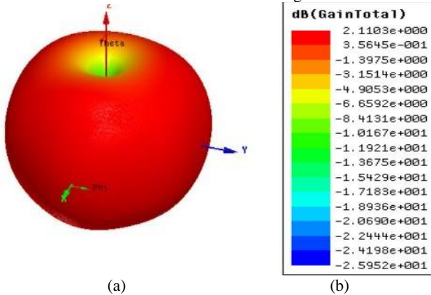
Fig. 5: a) 3D polar plot, b) Gain readings
