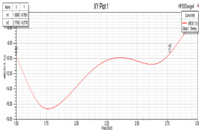
Fig. 6: Reflection coefficient
