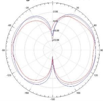
Fig.7: Radiation pattern
