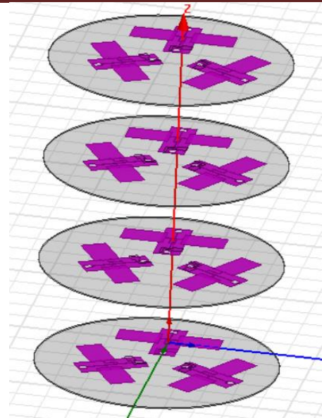
Fig. 8: Four antenna unit array
