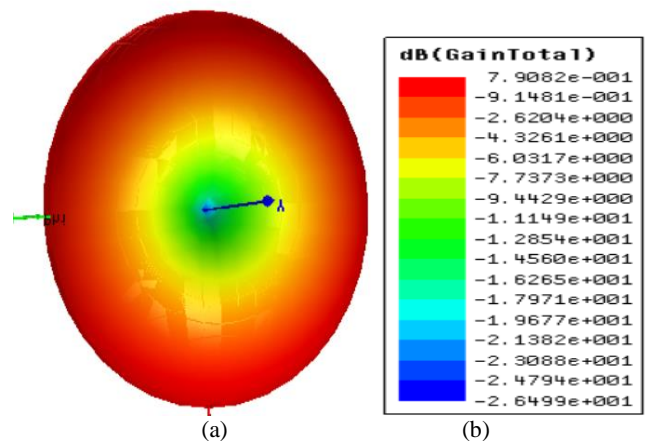
Fig.3: 3D polar plot, b) gain readings
