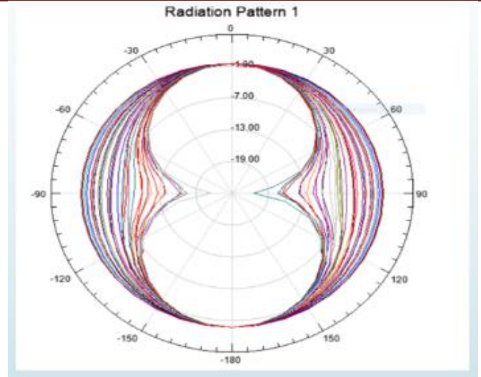
Fig.2 (b): Radiation pattern
