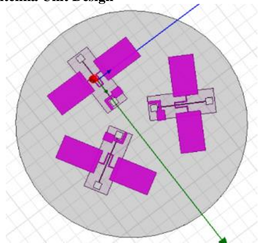
Fig.4: Antenna unit
