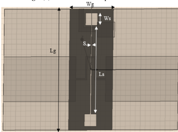
Fig.1 (b): Top view of dipole element
