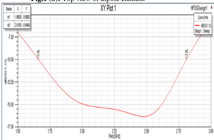
Fig.2 (a): Reflection coefficient graph
