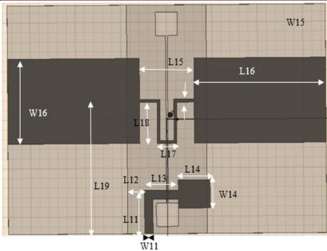
Fig.1 (a): Bottom view of dipole element
